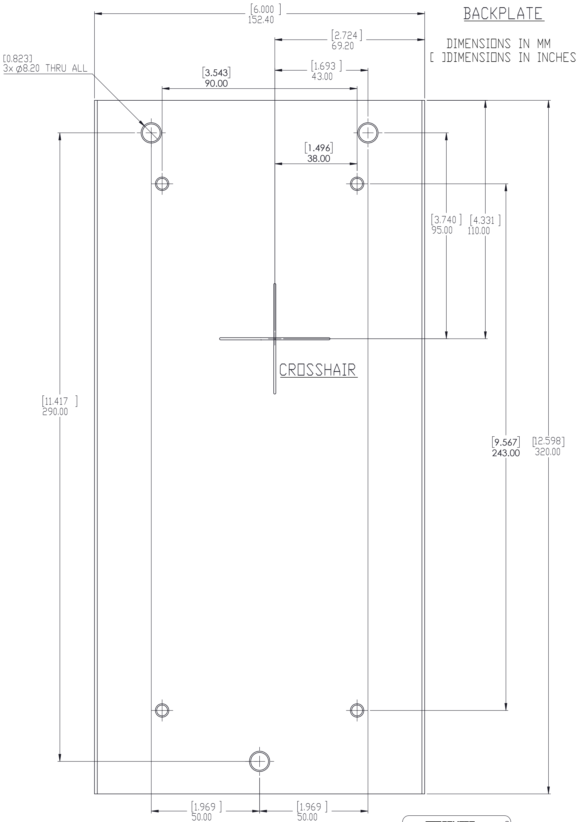
HOSPITAL GREEN LASER TEMPLATE TMPL-1504-23B(CR)
